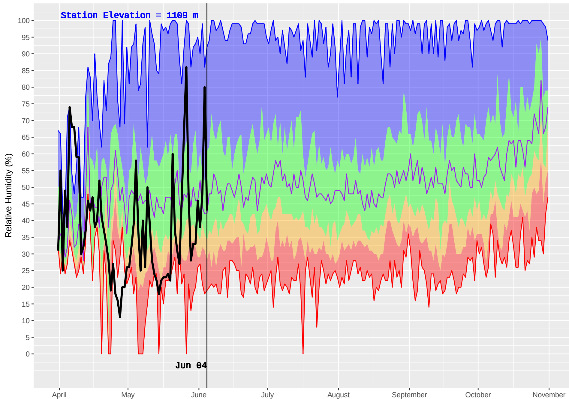
MOOSE LAKE (165) : Historical (1980–2016) and Current (2018) Noon Relative Humidity
